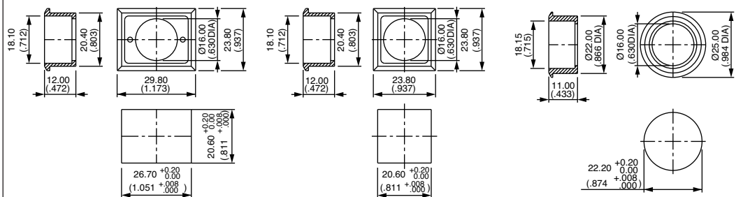
Round A01FM2
