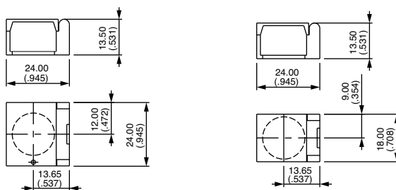
Square/round A01FG2
