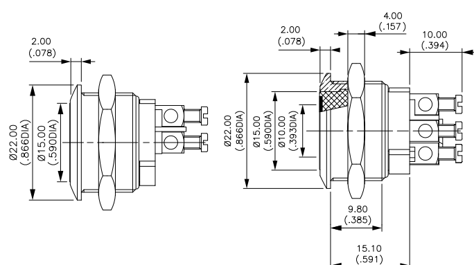
Hex nut 22 (.866) across flats
