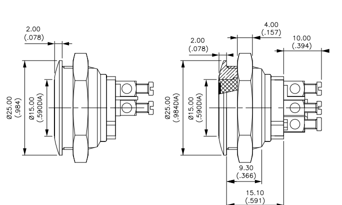
Hex nut 25 (.984) across flats
