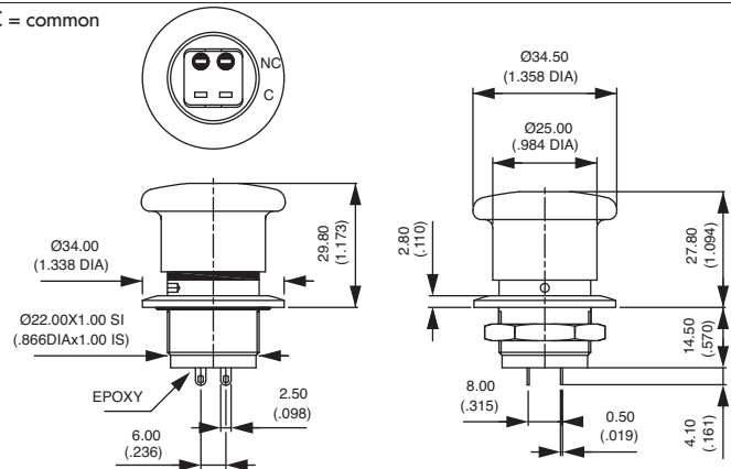
Shown with solder lug terminals
