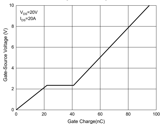
Fig. 6 - Gate Charge
