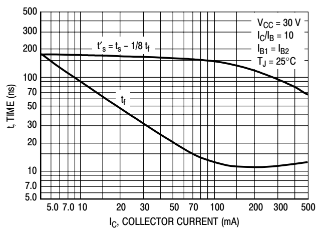
Figure 4. Turn-Off Time
