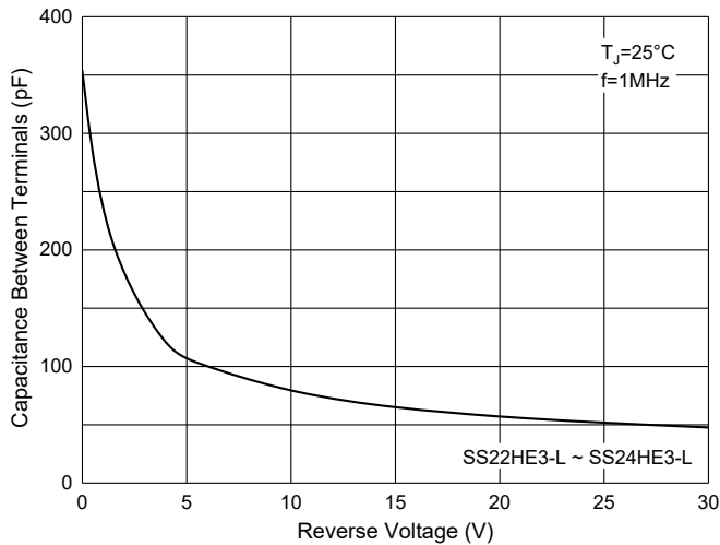
Fig. 9 - Capacitance Characteristics
