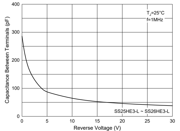
Fig. 10 - Capacitance Characteristics
