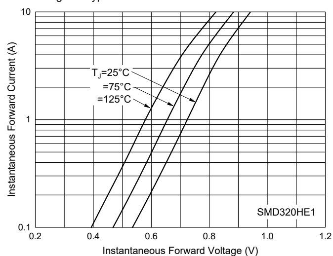
Fig. 9 - Typical Instantaneous Forward Characteristics
