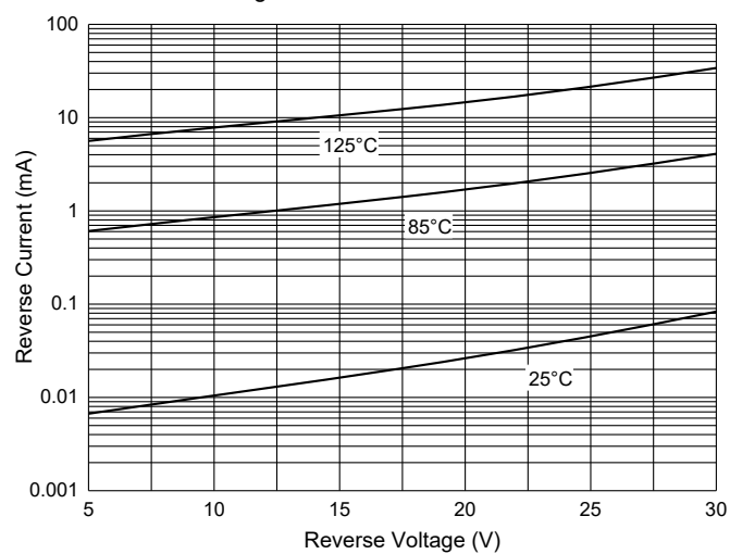
Fig. 4 - Reverse Characteristics
