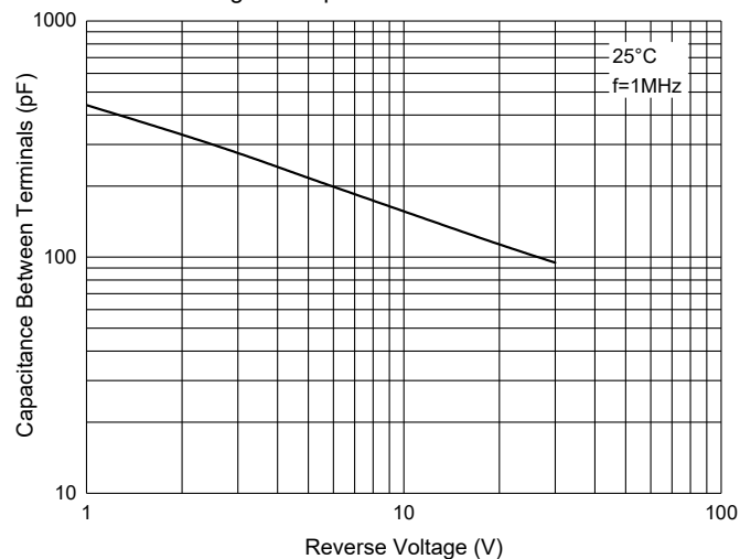
Fig. 2 - Capacitance Characteristics
