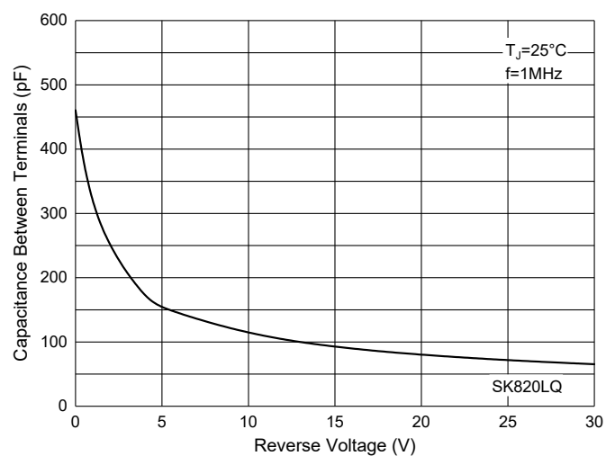
Fig. 8 - Capacitance Characteristics
