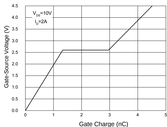
Fig.6 - Gate Charge
