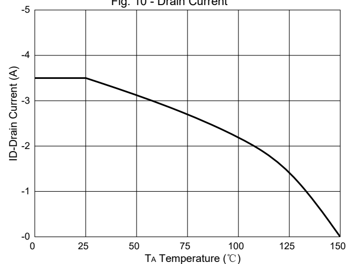
Fig. 10 - Drain Current
