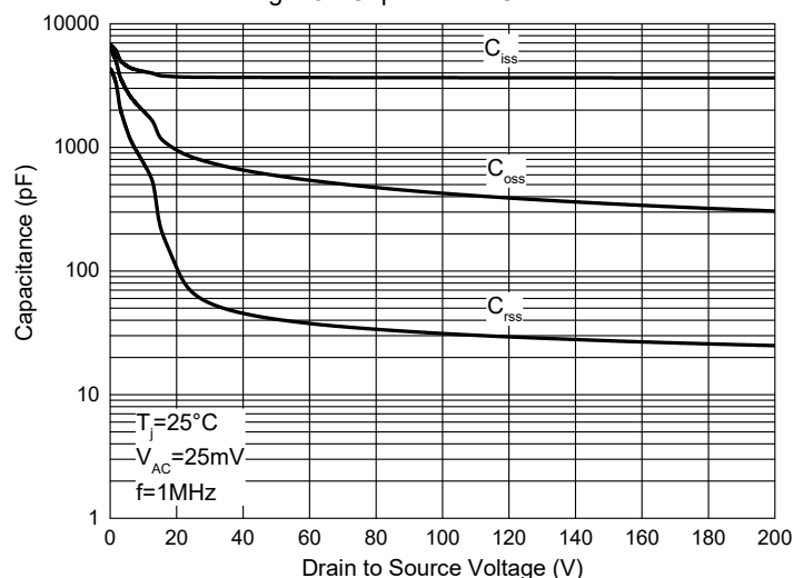
Fig. 13 - Capacitance Characteristics
