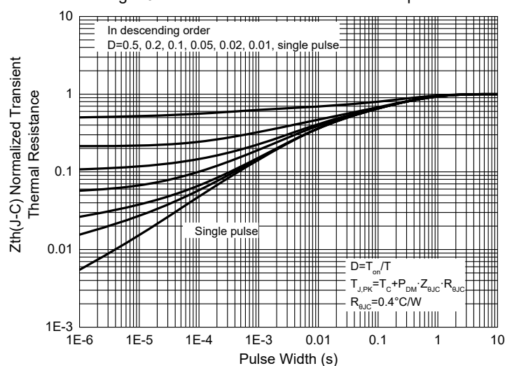
Fig. 16 - Normalized Transient Thermal Impedance
