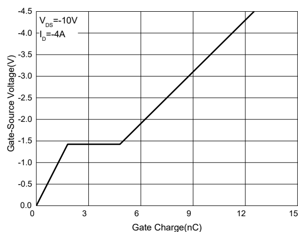
Fig.6 - Gate Charge
