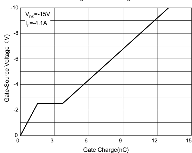
Fig. 6 - Gate Charge
