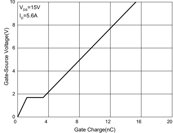
Fig.6 - Gate Charge
