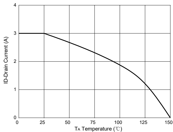
Fig. 10 - Drain Current
