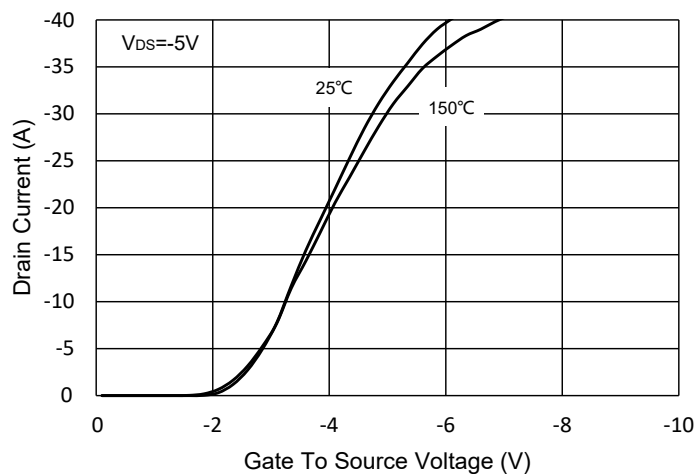
Fig.2 - Transfer Characteristic
