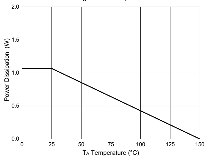
Fig.11-PD Dissipation
