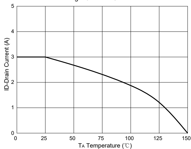
Fig. 10 - Drain Current
