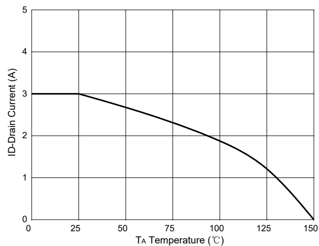
Fig. 10 - Drain Current
