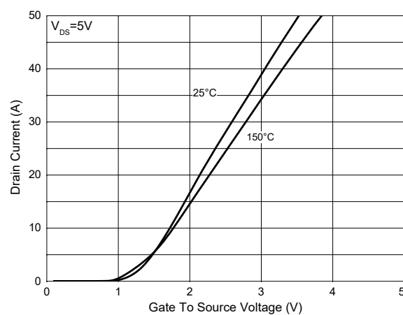
Fig. 2 - Transfer Characteristics
