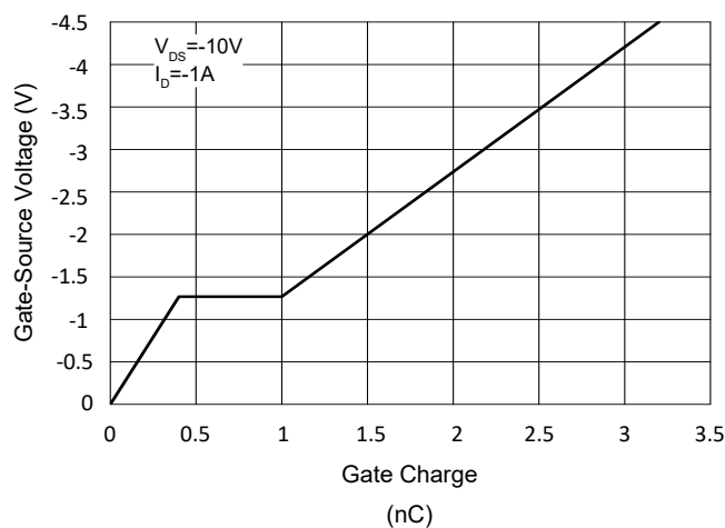
Fig.6 - Gate Charge
