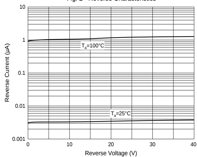
Fig. 2 - Reverse Characteristics
