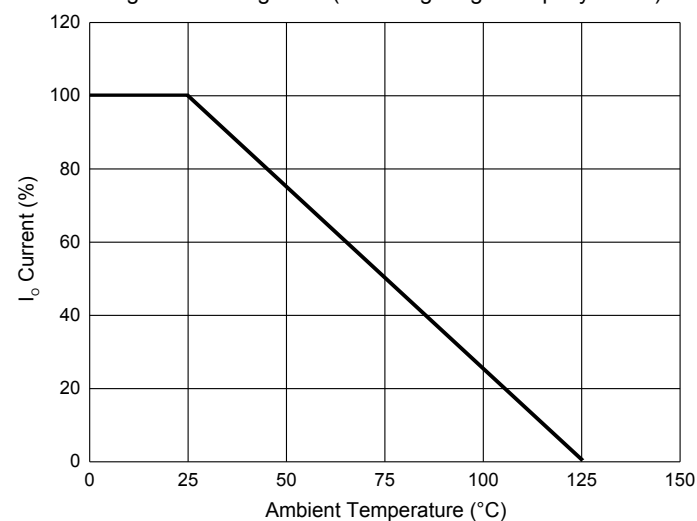
Fig. 4 - Derating curve(mounting on glass epoxy PCBs)
