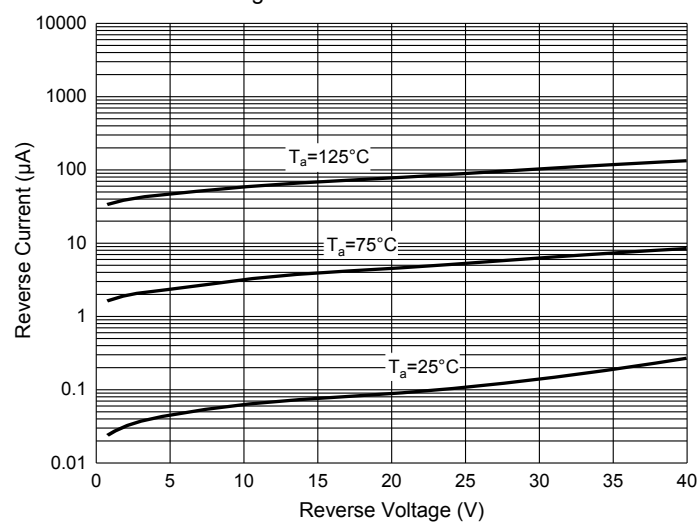
Fig. 2 - Reverse Characteristics
