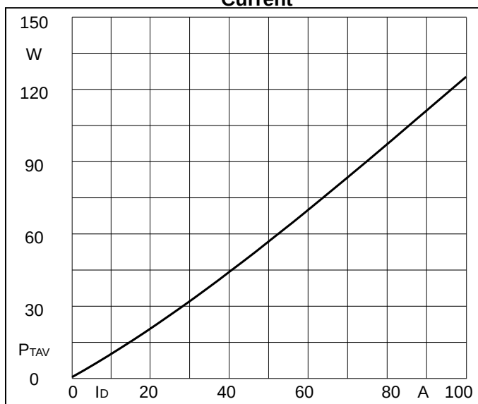
Fig6. SCR Power dissipation
