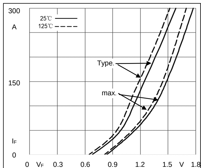
Fig5. Diode Forward Characteristics
