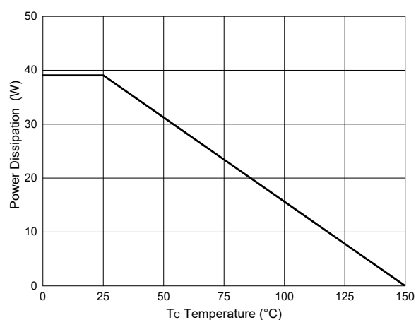
Fig.11 Power Dissipation
