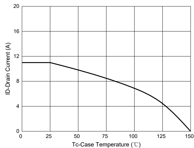
Fig. 10 - Current dissipation
