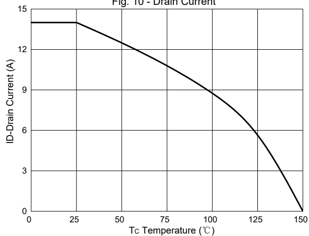
Fig. 10 - Drain Current
