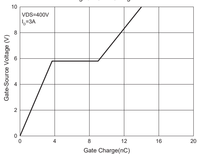
Fig. 6 - Gate Charge
