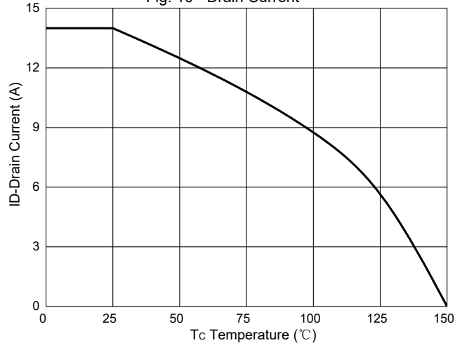
Fig. 10 - Drain Current
