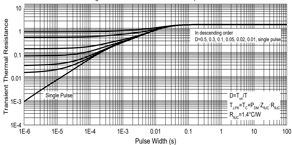
Fig.8 - Maximum Transient Thermal Impedance
