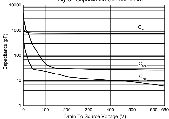
Fig. 6 - Capacitance Characteristics
