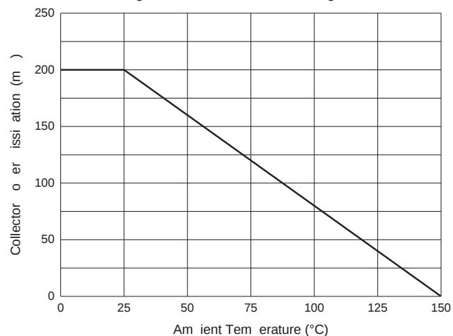
Fig. 6 - Collector Power Dissipating Current
