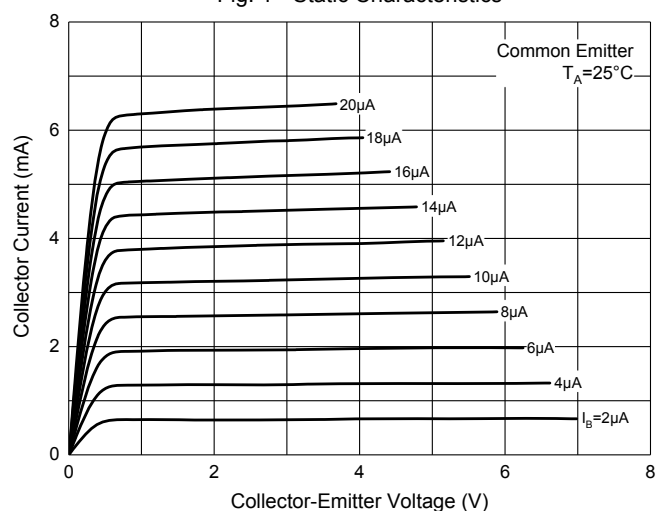
Fig. 1 - Static Characteristics
