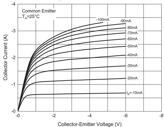
Fig. 1 - Static Characteristics
