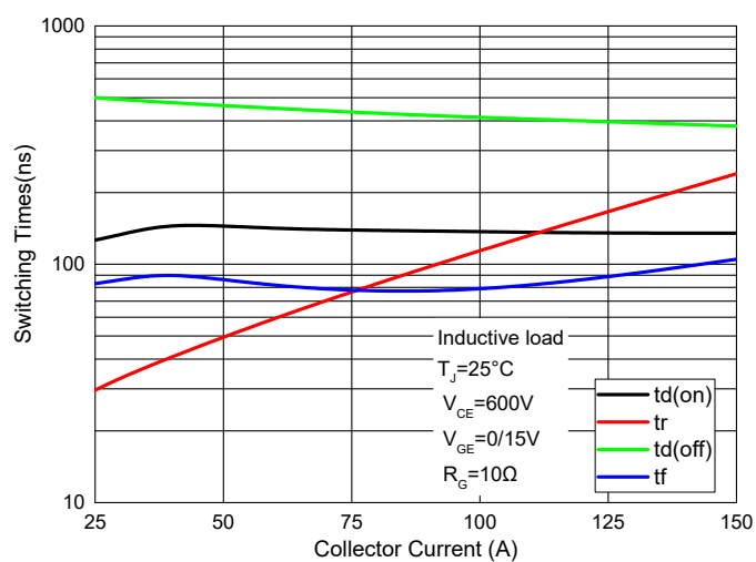
Fig. 9 - Switching Times — I_C
