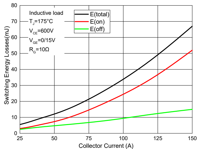
Fig. 12 - Switching Energy Losses — I_C
