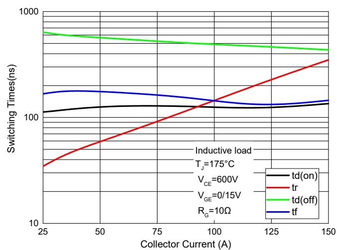
Fig. 10 - Switching Times — I_C
