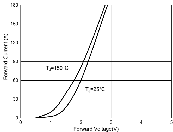
Fig. 7 - Forward Voltage
