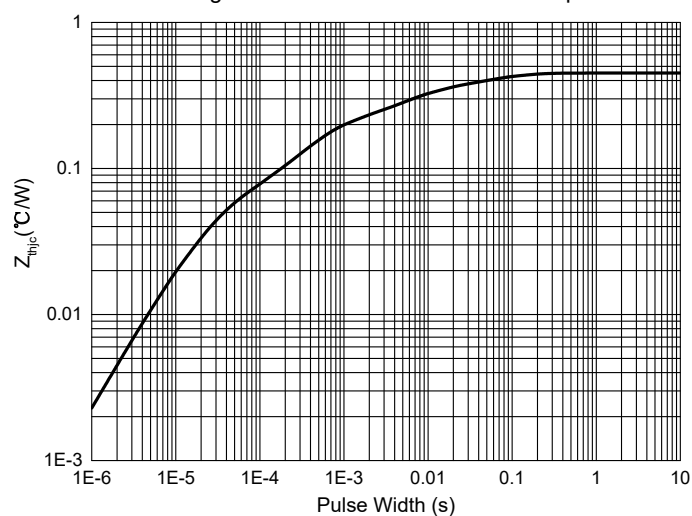
Fig. 22 - Diode Transient Thermal Impedance
