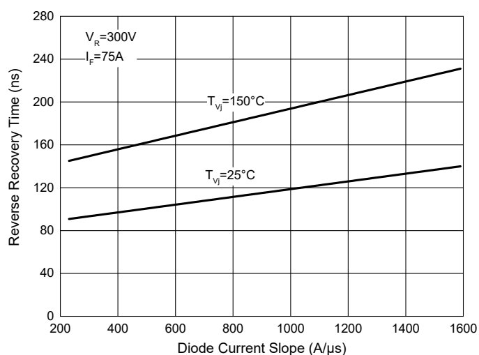
Fig. 18 - Typical T_{rr} vs Diode Current Slope
