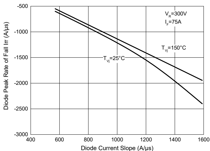
Fig. 16 - Typical di_{rr}/dt vs Diode Current Slope
