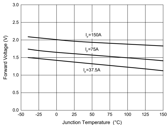
Fig. 20 - V_F vs Junction Temperature
