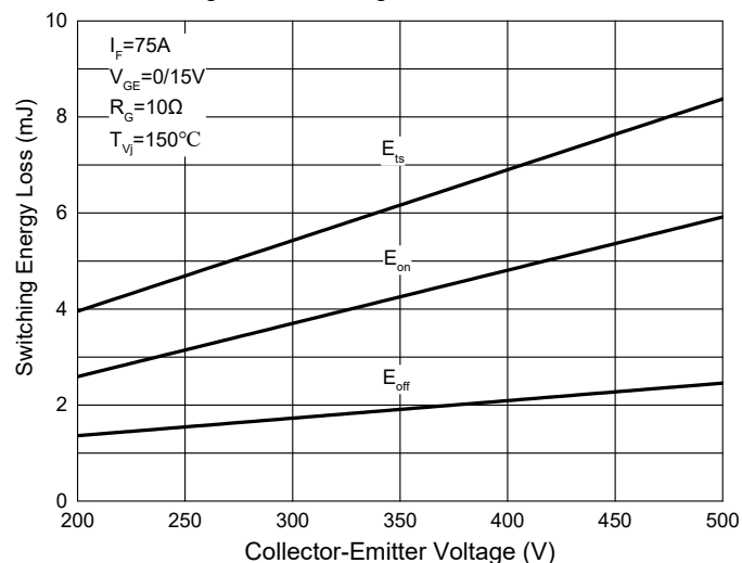
Fig. 10 - Switching Loss vs V_{CE}
