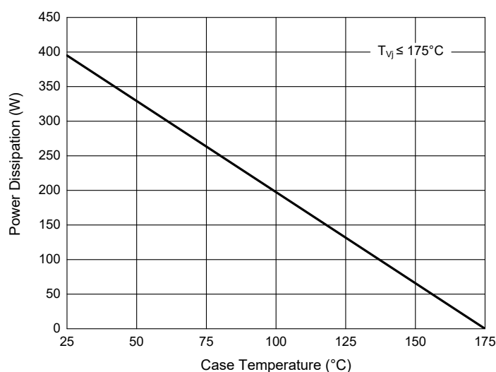
Fig. 24 - Power Derating
