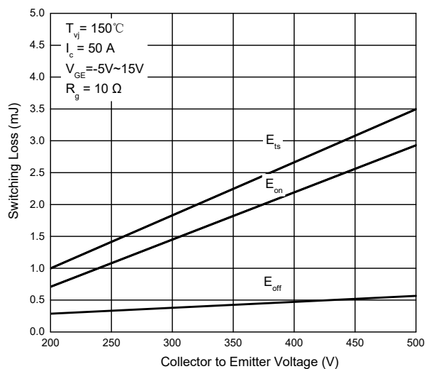
Fig. 10 -IGBT Switching Loss vs. V_{CE}
