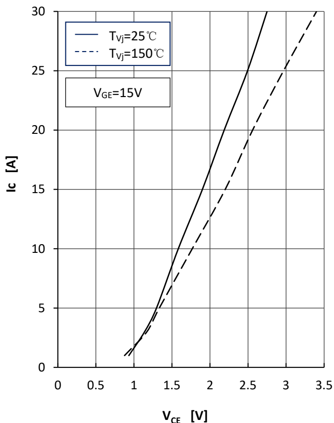
Fig1.IGBT Output Characteristics
