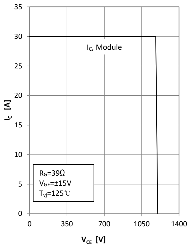
Fig5. RBSOA
