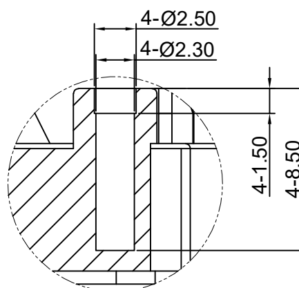
View C scale 4:1
