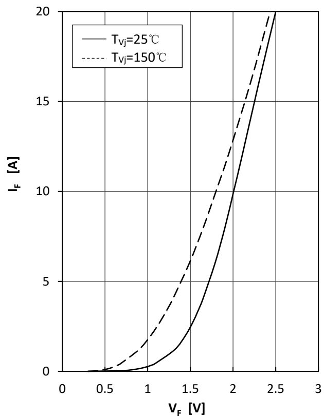
Fig13.Diode-brake-chopper Forward Characteristics
