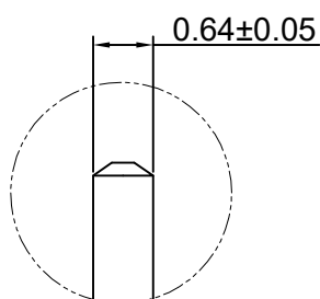
View B scale 4:1
