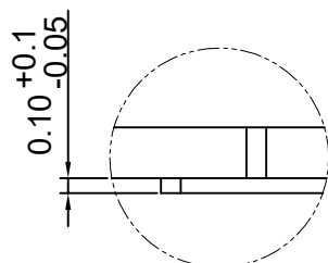
View A scale 4:1
