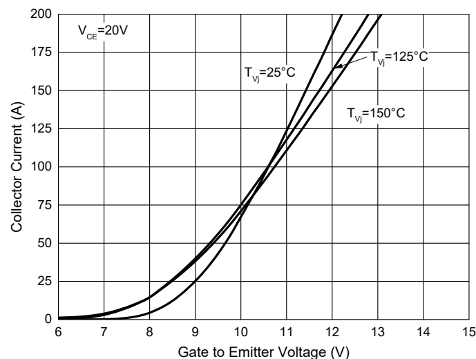
Fig. 2 - IGBT Transfer Characteristics
