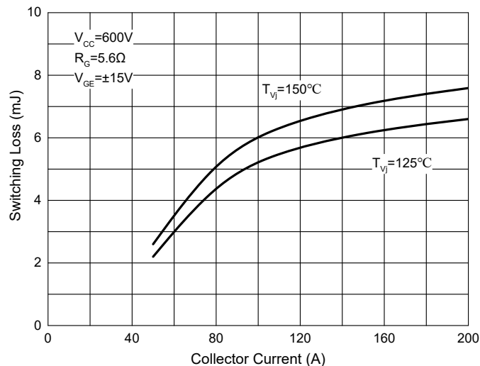
Fig. 8 - Diode Switching Loss ( E_{rec} ) vs IF
