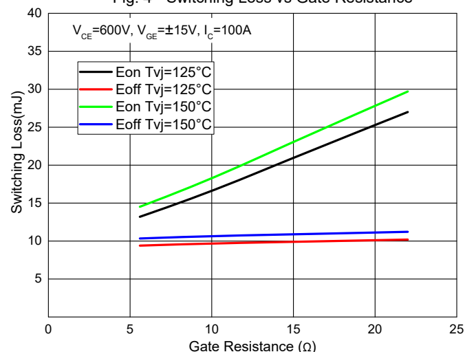
Fig. 4 - Switching Loss vs Gate Resistance
