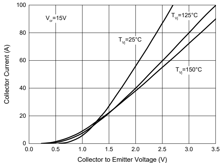
Fig. 12 - IGBT-brake-Chopper Output Characteristics
