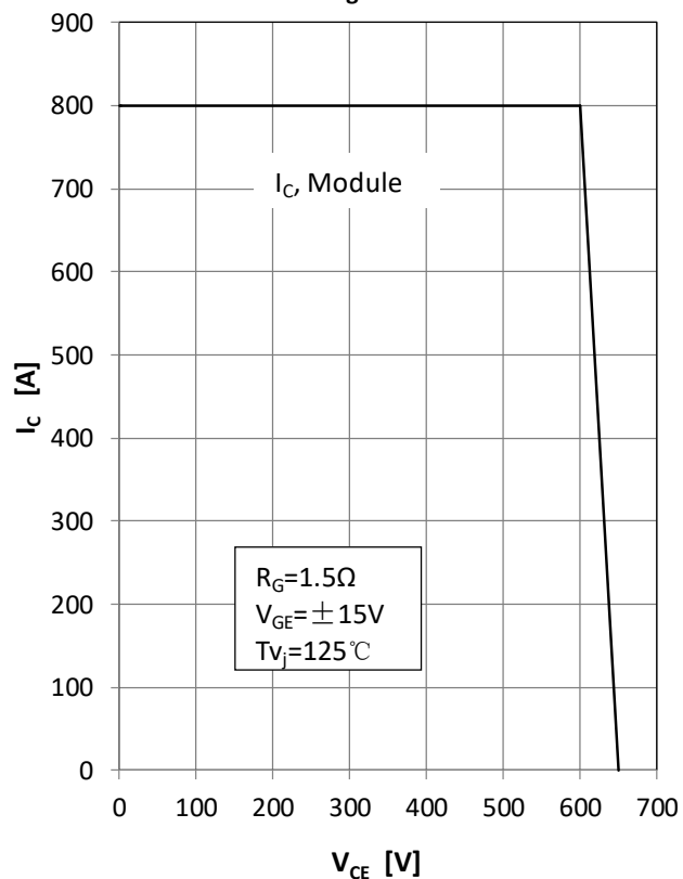
Fig5. RBSOA
