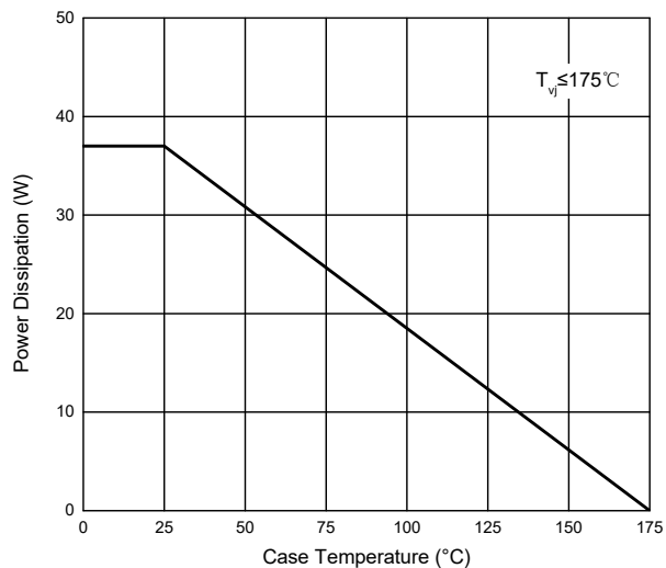
Fig. 11 - Power Derating
