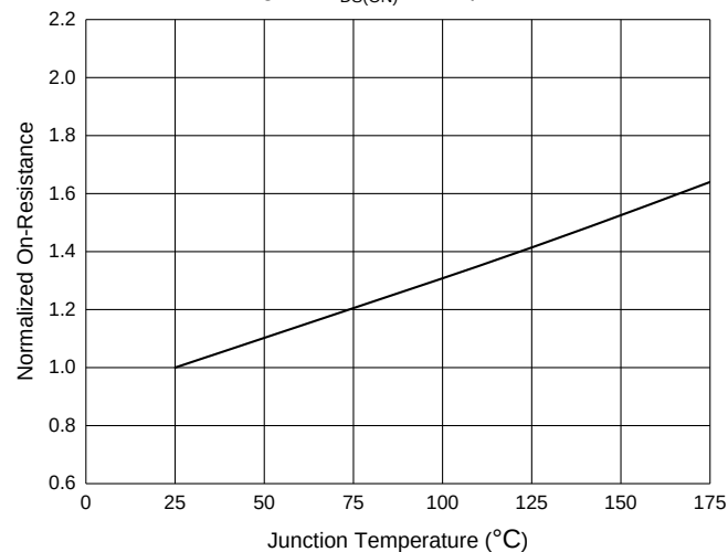
Fig. 6 - R_{DS(ON)} - \text{Temperature}
