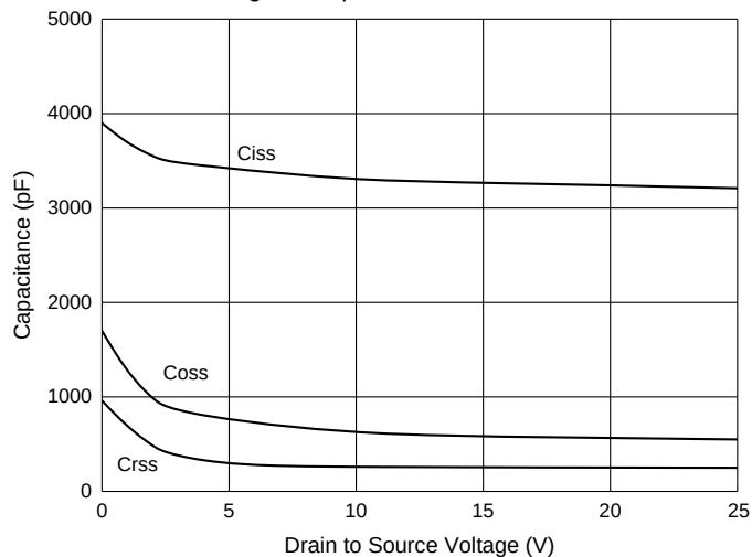
Fig. 3 - Capacitance Characteristics
