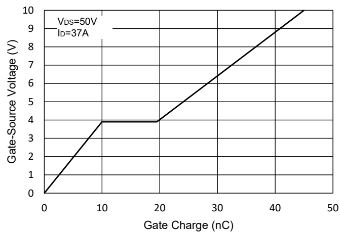
Fig.6 - Gate Charge
