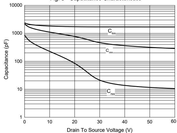
Fig. 5 - Capacitance Characteristics
