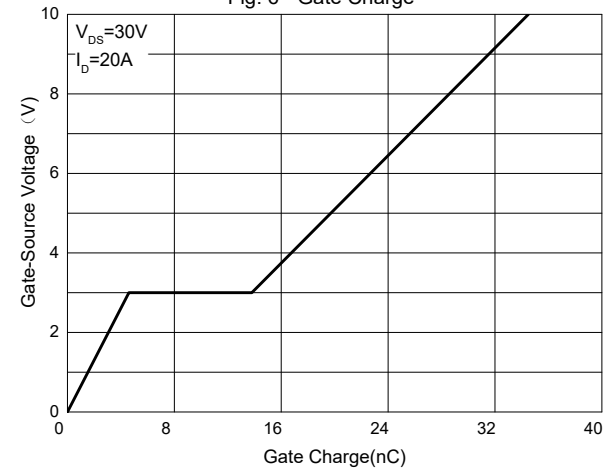
Fig. 6 - Gate Charge
