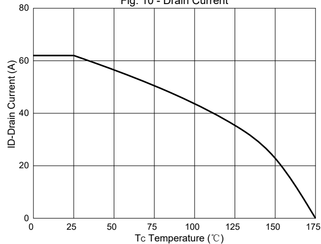
Fig. 10 - Drain Current
