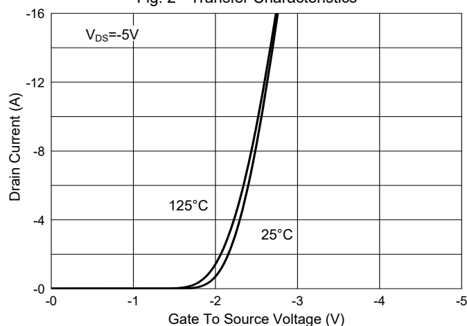
Fig. 2 - Transfer Characteristics
