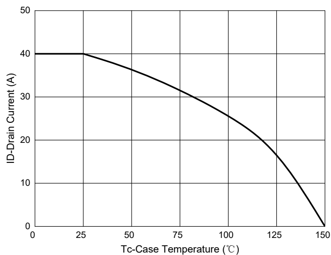
Fig. 10 - Current dissipation
