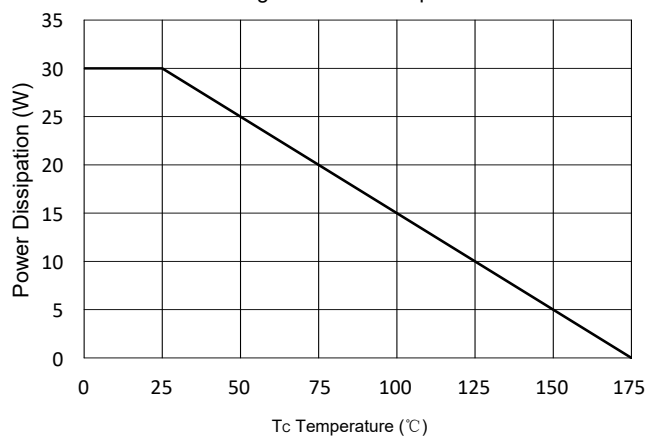
Fig.11 Power Dissipation
