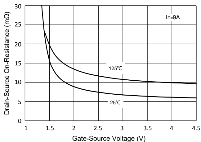
Fig.3 Rds(on)-Vgs
