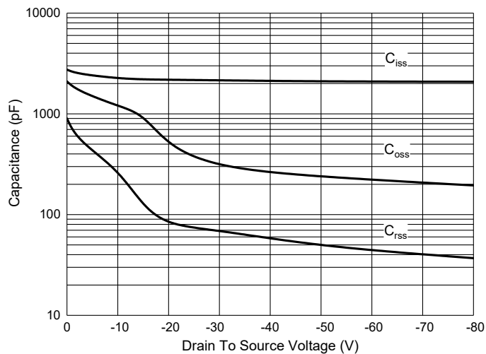
Fig. 7 - Capacitance Characteristics
