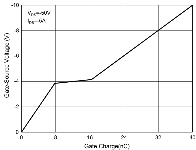
Fig. 8 - Gate Charge
