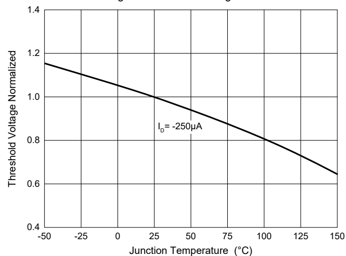
Fig. 8 - Threshold Voltage
