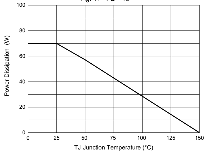
Fig. 11 - P_D - T_J
