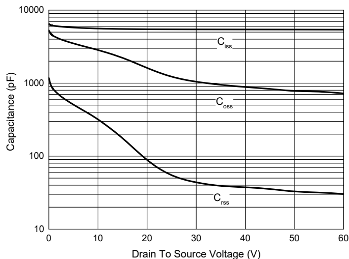
Fig. 7 - Capacitance Characteristics
