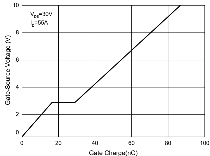
Fig. 8 - Gate Charge
