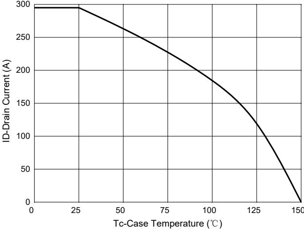
Fig. 10 - Current dissipation
